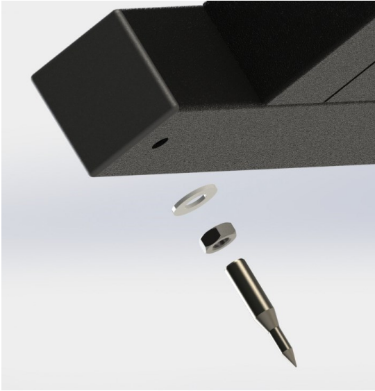
SPIKE ASSEMBLY
